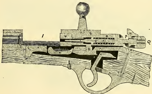
The Mauser Rifle.
